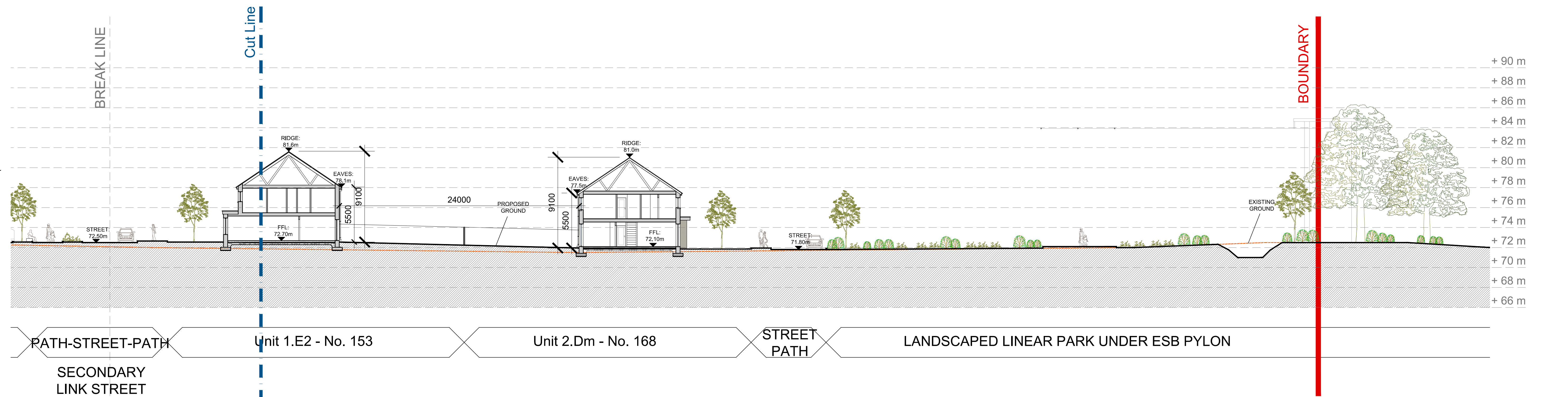
PROPOSED SITE SECTION AA (Part 2) - scale 1:200
